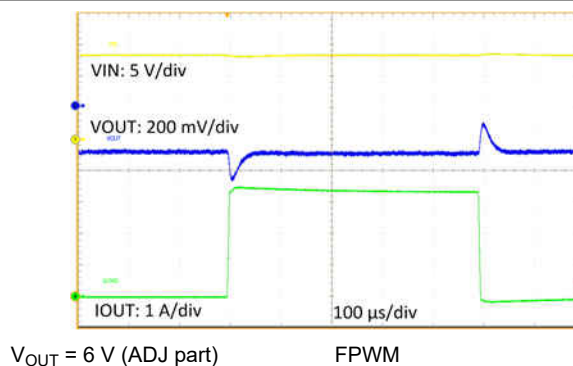
Figure 9-38. Load Transient
