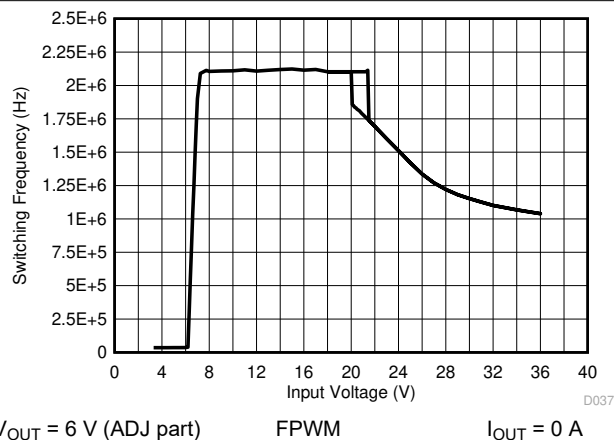
Figure 9-35. Switching Frequency vs Input Voltage
