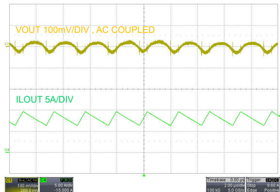
Figure 7-9. Output Ripple, V_{SUPPLY} = 48V , I_{LOAD} = 8A
