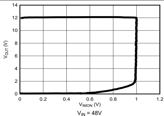
Figure 5-18. Constant-Current Constant-Voltage Operation During a Charing Transient
