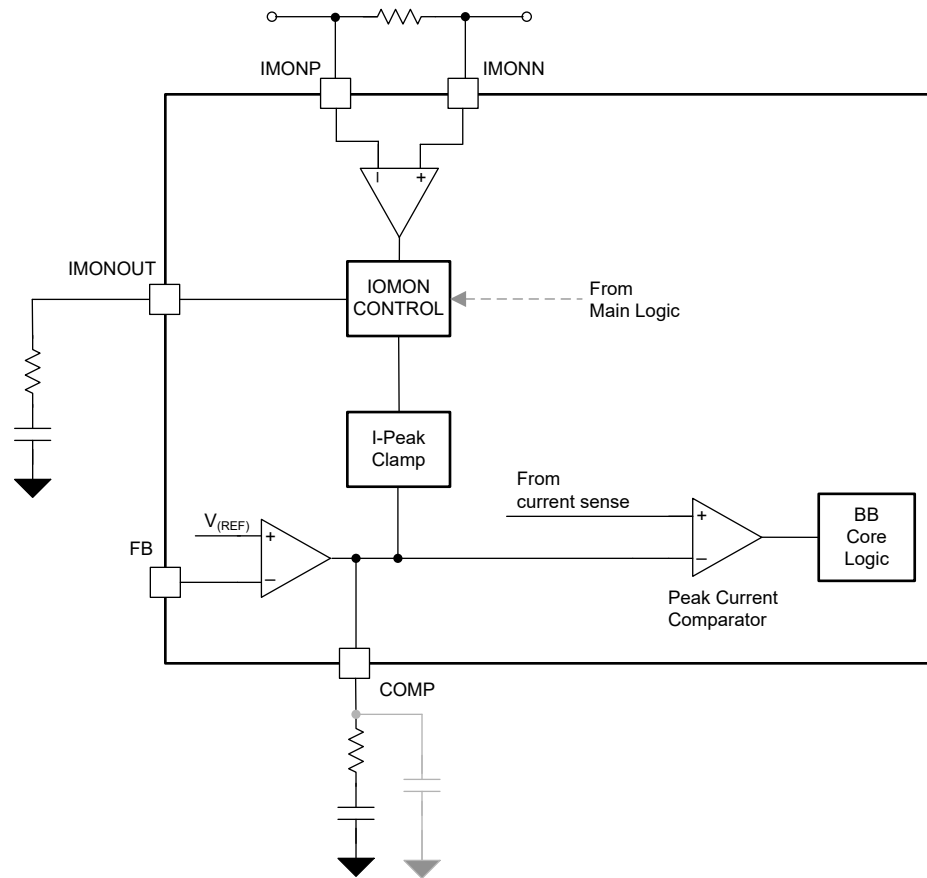
8.3.14 Short Circuit - Hiccup Protection
