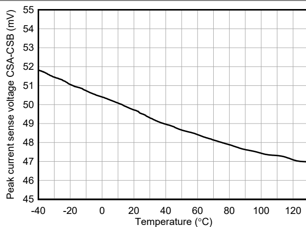
Figure 6-8. LM51770 Current Limit Threshold Voltage vs Temperature
