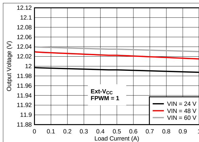
Figure 26. Load Regulation
