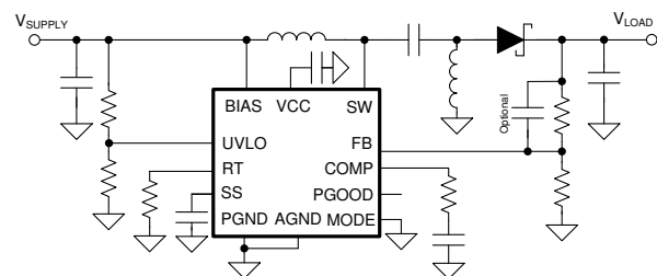
Typical SEPIC Application
