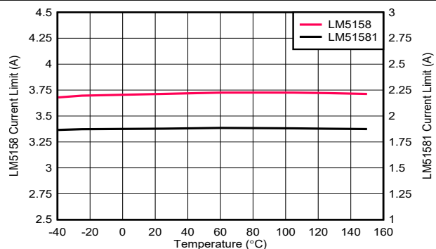
Figure 8-12. Current Limit Threshold vs Temperature
