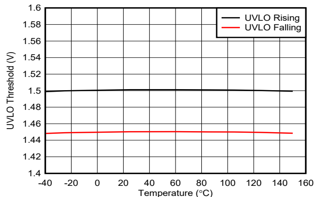
Figure 8-8. UVLO Threshold vs Temperature
