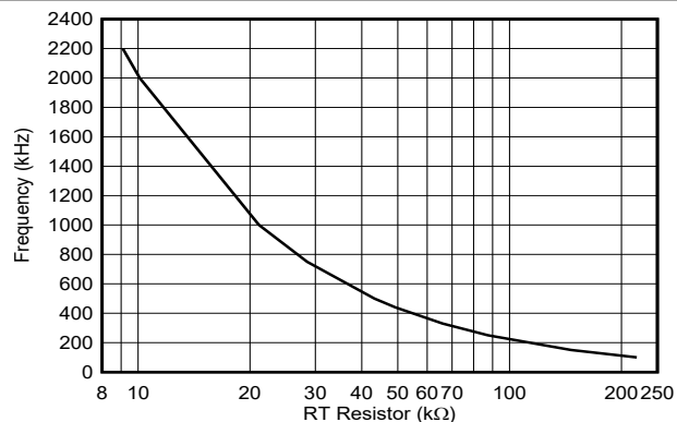
Figure 8-10. Frequency vs RT Resistance
