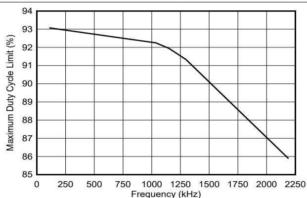
Figure 8-16. Maximum Duty Cycle Limit vs Frequency
