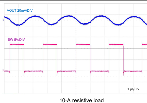
Figure 9-31. Full Load Switching
