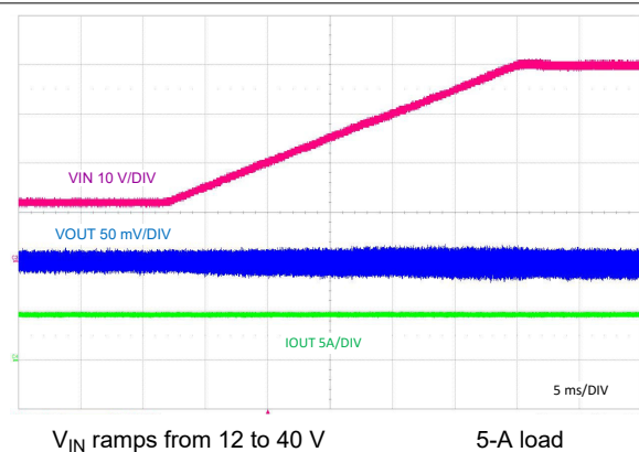
Figure 9-33. Line Transient Response to V_{IN} = 40 V
