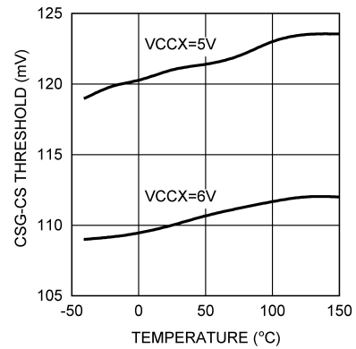
Figure 5-18. Current Limit Threshold vs Temperature
