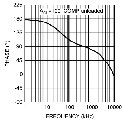
Figure 5-16. Error Amp Phase vs Frequency
