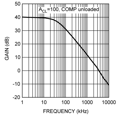
Figure 5-14. Error Amp Gain vs Frequency
