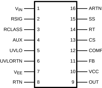
Figure 2. 16 Lead TSSOP
