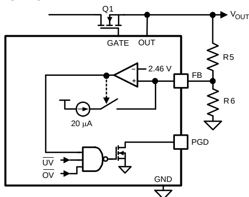
Figure 33. Programming the PGD Threshold
