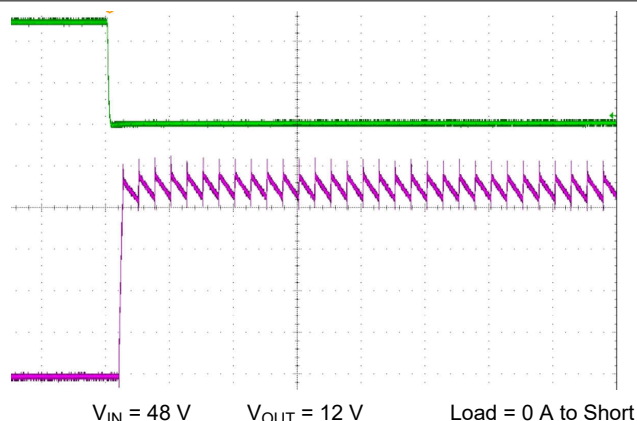
Figure 9-7. Short Circuit Applied
