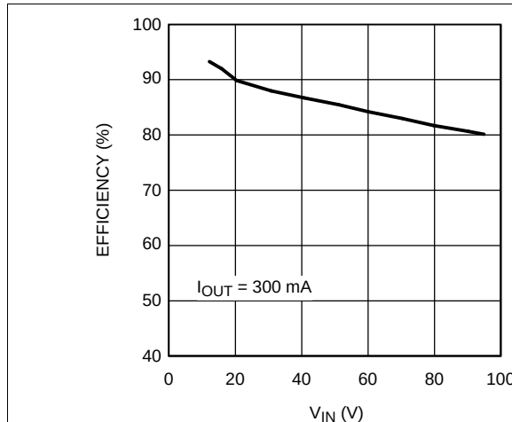
Figure 12. Efficiency vs V IN
