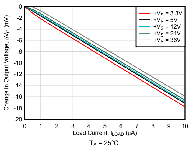
Figure 6-28. Change in Output Voltage vs Load Current
