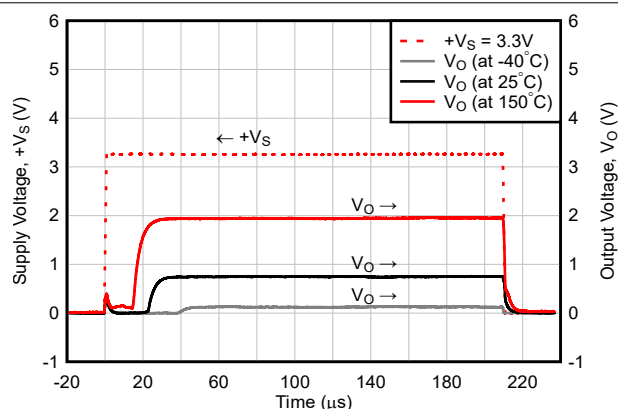
Figure 6-30. Start-up response to +V_S = 3.3\text{V} Step (When t_r = 1\mu\text{s} , No C_{\text{Load}} and C_{\text{By-pass}} )
