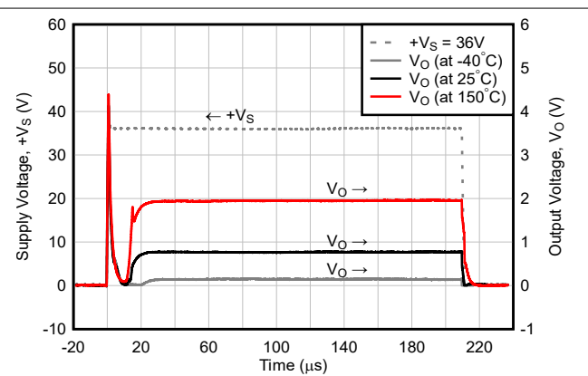
Figure 8-5. Start-up Response to +V_S = 36V Step (When t_r = 1\mu s , No C_{Load} and C_{By-pass} )
