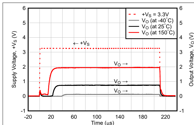
Figure 8-4. Start-up response to +V_S = 3.3V Step (When t_r = 1\mu s , No C_{Load} and C_{By-pass} )
