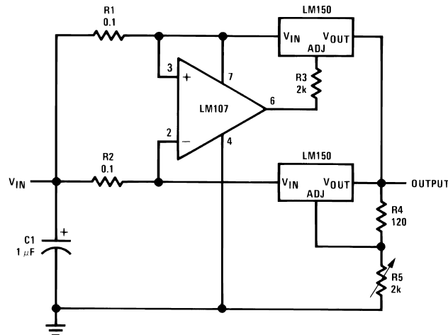
Figure 43. 6A Regulator
