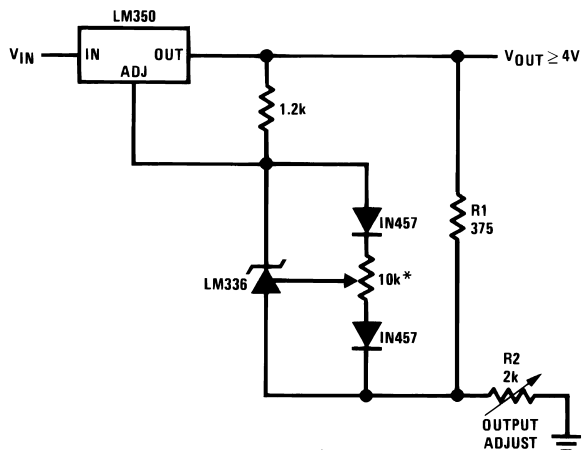
Figure 20. Precision Power Regulator with Low Temperature Coefficient
