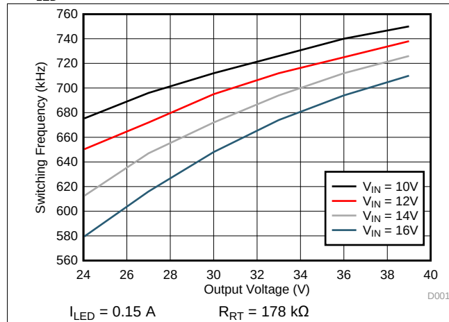
Figure 17. Switching Frequency vs Output Voltage
