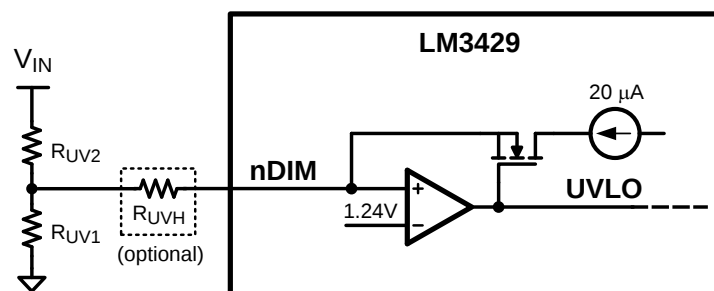
Figure 23. UVLO Circuit
