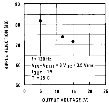
Figure 6. Ripple Rejection
