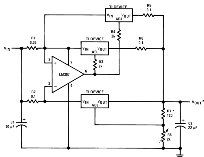
Figure 30. 15-A Regulator
