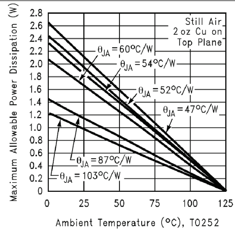
Figure 40. Maximum Allowable Power Dissipation vs Ambient Temperature for TO-252
