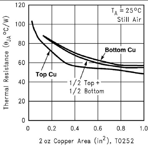
Figure 39. \theta_{JA} vs 2-oz. Copper Area for TO-252
