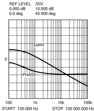
Figure 7-4. Gain and Phase of Modulator R_{\text{LOAD}} = 5 \text{ Ohms} and C_{\text{OUT}} = 130 \mu\text{F}
