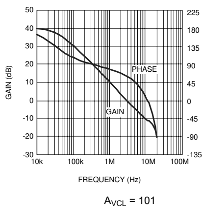
Figure 5-5. Error Amplifier Gain and Phase
