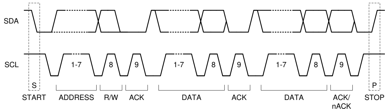
Figure 8-34. I 2 C START / STOP / ACKNOWLEDGE Protocol
