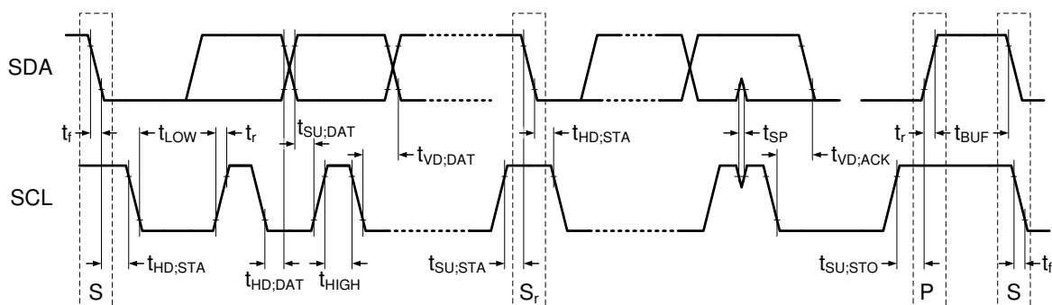
Figure 8-35. I 2 C Data Transmission Timing
