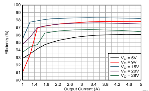
Efficiency vs. Output Current, V_1 = 12\text{V} , PSM
