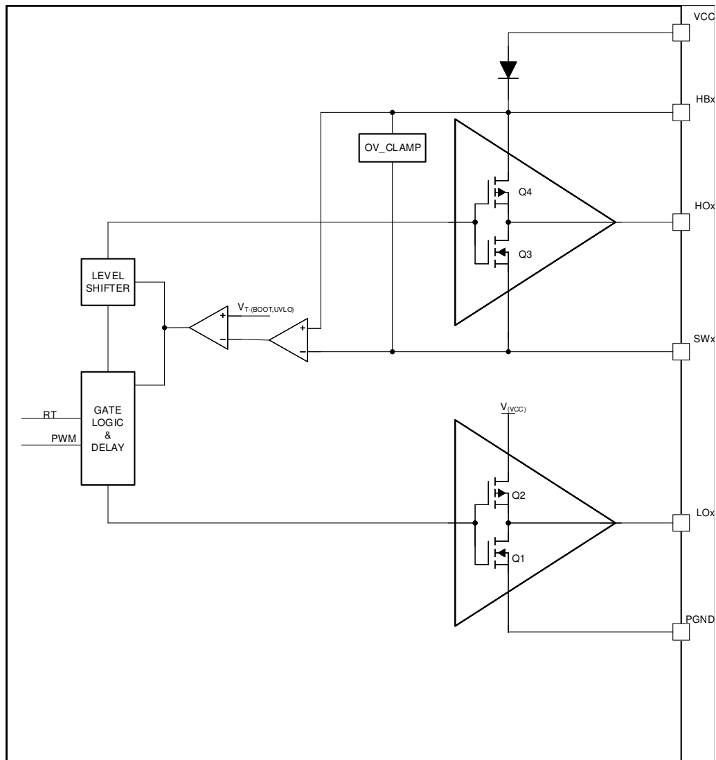
Figure 8-28. Functional Block Diagram Gate Driver
