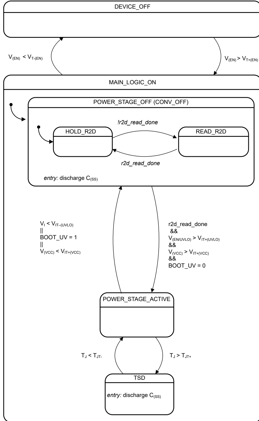
Figure 8-33. State Diagram
