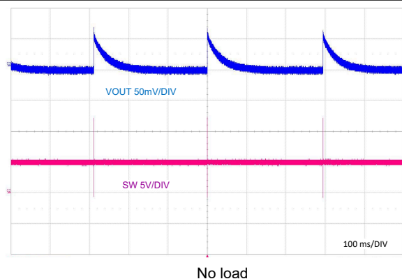
Figure 9-22. PFM Switching
