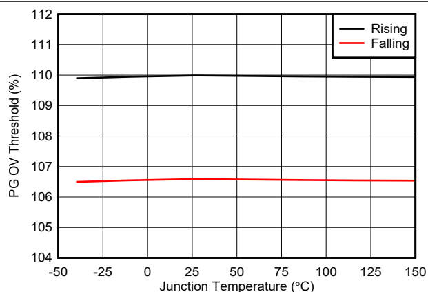
Figure 7-10. PG OV Thresholds vs. Temperature
