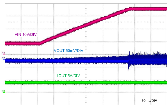
Figure 9-7. Full Load Switching
