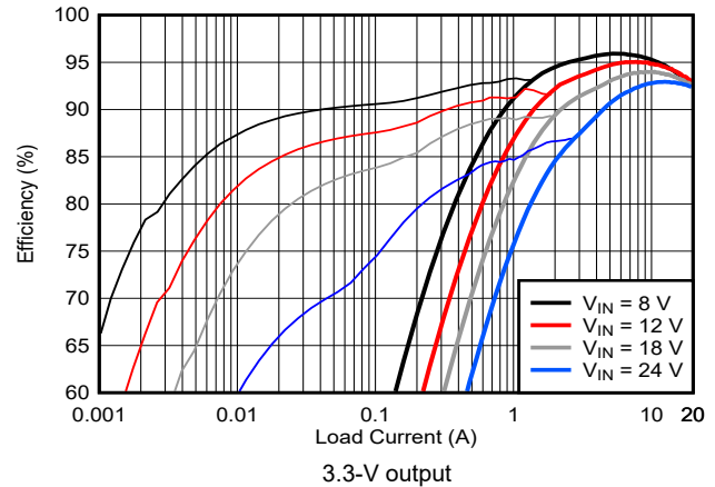
Figure 9-30. Efficiency vs I_{OUT} , Log Scale
