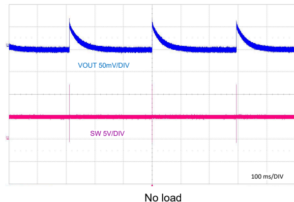
Figure 9-21. PFM Switching
