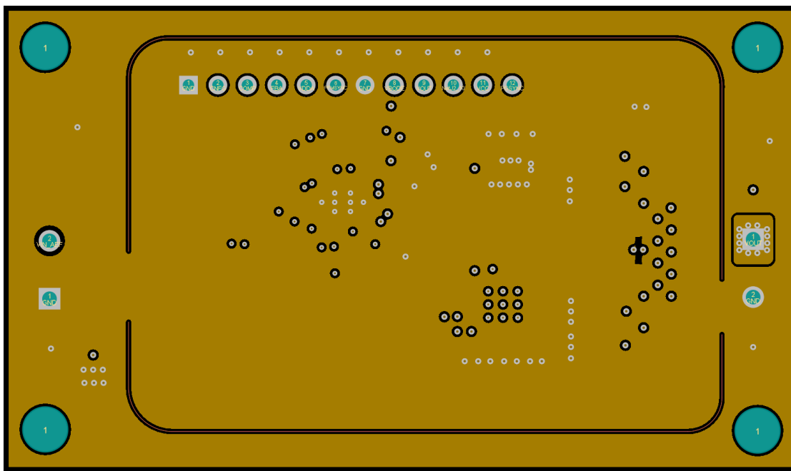
Figure 11-3. Layer 2 Full Ground Plane Directly Under the Power Components
