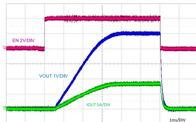
V_{IN} = 12 V 8-A resistive load Figure 9-12. ENABLE ON and OFF Characteristic
