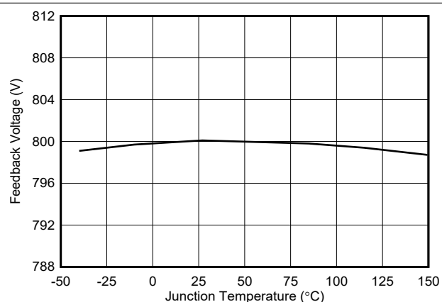
Figure 7-9. Feedback Voltage vs. Temperature
