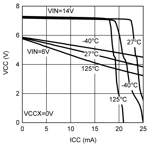
Figure 5-23. VCC vs ICC
