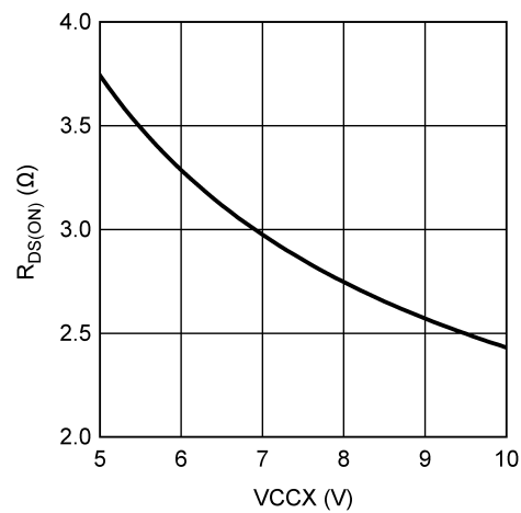
Figure 5-24. VCCX Switch R_{DS(ON)} vs VCCX
