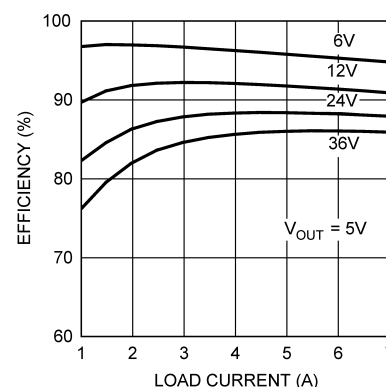
Typical Application Circuit Efficiency
