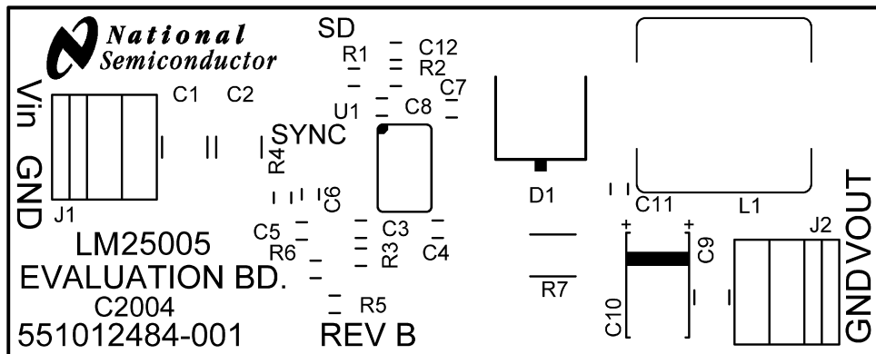
Figure 7-10. Silkscreen
