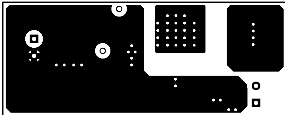
Figure 7-9. Solder Side
