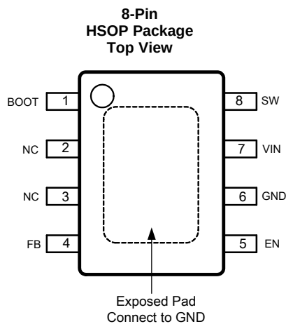
Pin Functions
