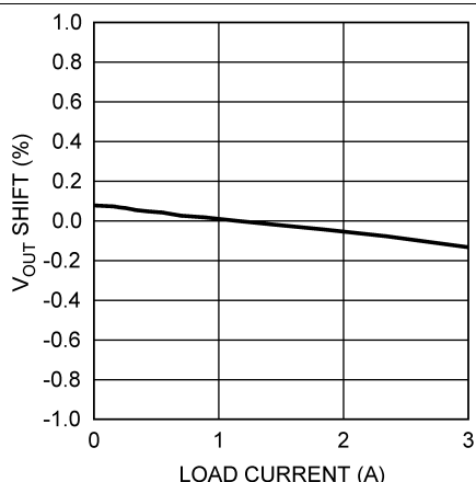
Figure 11. Load Regulation
