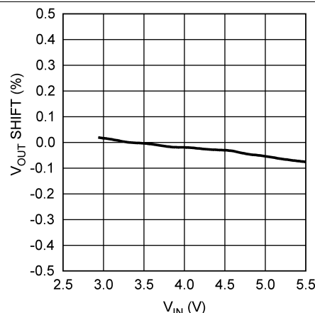
Figure 10. Line Regulation
