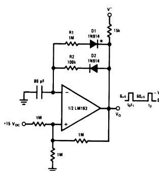
Pulse Generator
