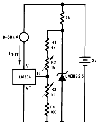
Figure 17. 0°F–50°F Thermometer
