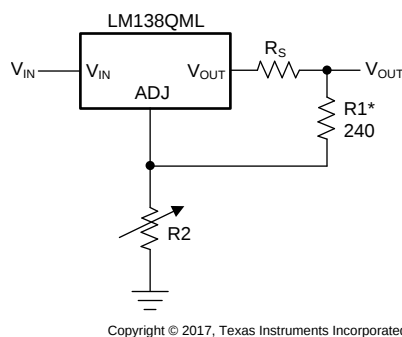
Figure 16. Regulator With Line Resistance in Output Lead
