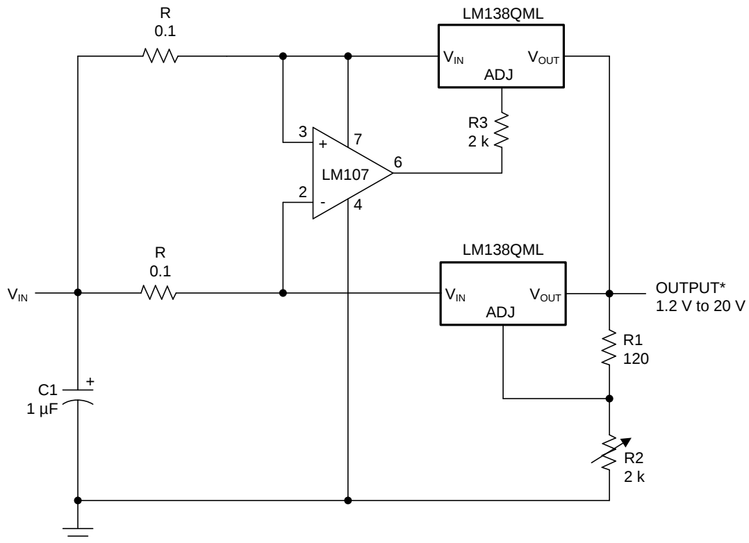
Figure 43. 10-A Regulator
