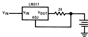
Figure 9-20. 50-mA Constant Current Battery Charger
