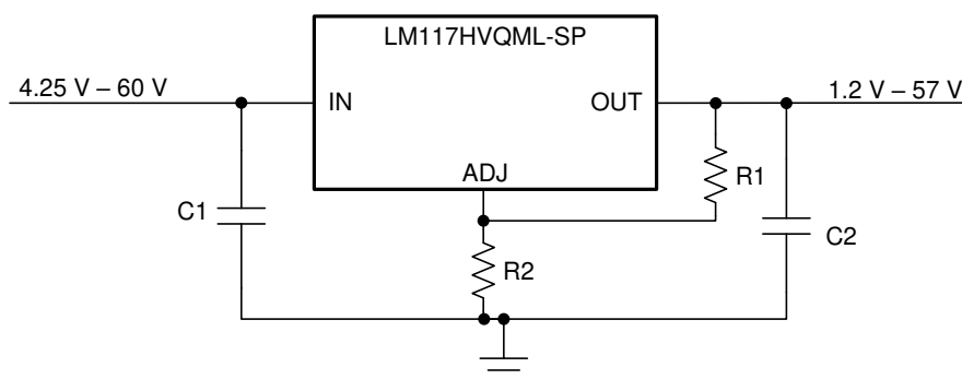
Simplified Schematic
