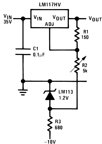
Figure 9-8. 0-V to 30-V Regulator
