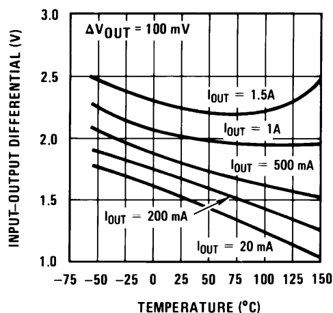
Figure 7-4. Dropout Voltage
