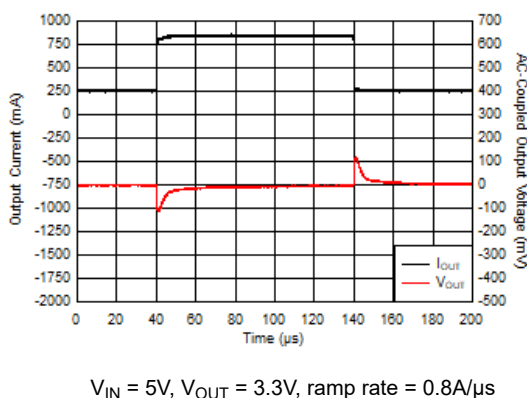
Figure 7-6. I_{OUT} Transient From 250mA to 850mA
