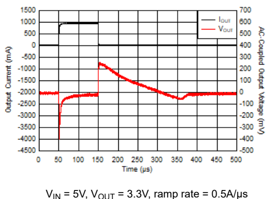
Figure 7-5. I_{OUT} Transient From 1mA to 1A
