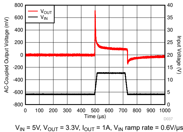
Figure 5-9. V_{IN} Transient in Dropout From 4V to 13V
