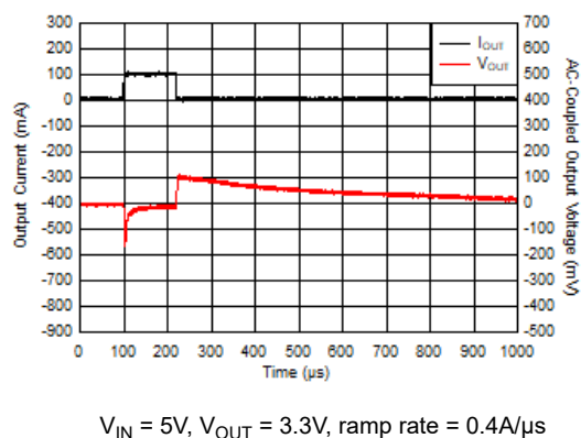
Figure 7-4. I_{OUT} Transient From 0mA to 100mA
