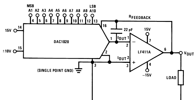
Figure 25. 10-Bit Linear DAC with No V_{OS} Adjust
