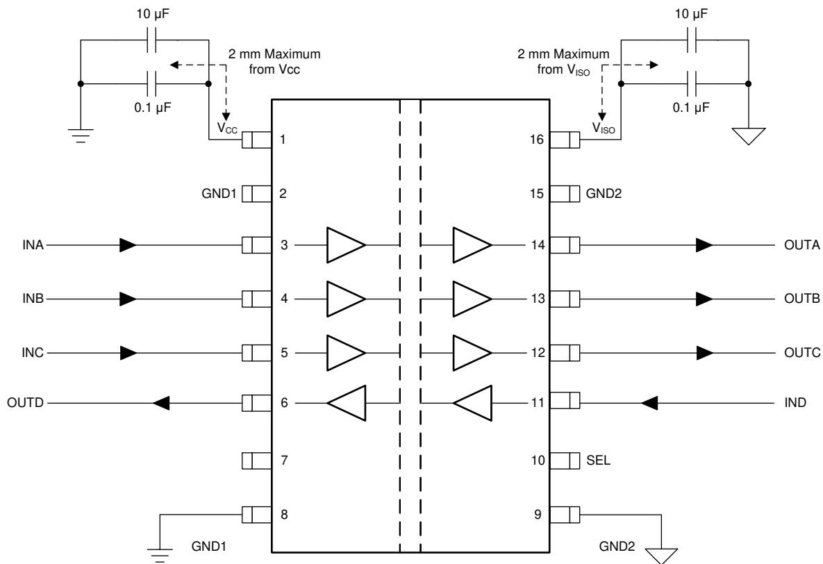
Figure 10-2. Typical ISOW7841A-Q1 Circuit Hook-Up
