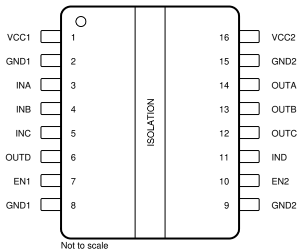
Figure 4-1. ISOS141-SEP DBQ Package 16-pin QSOP Top View
