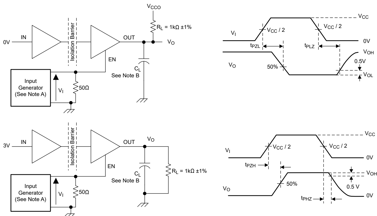
Figure 7-1. Switching Characteristics Test Circuit and Voltage Waveforms
