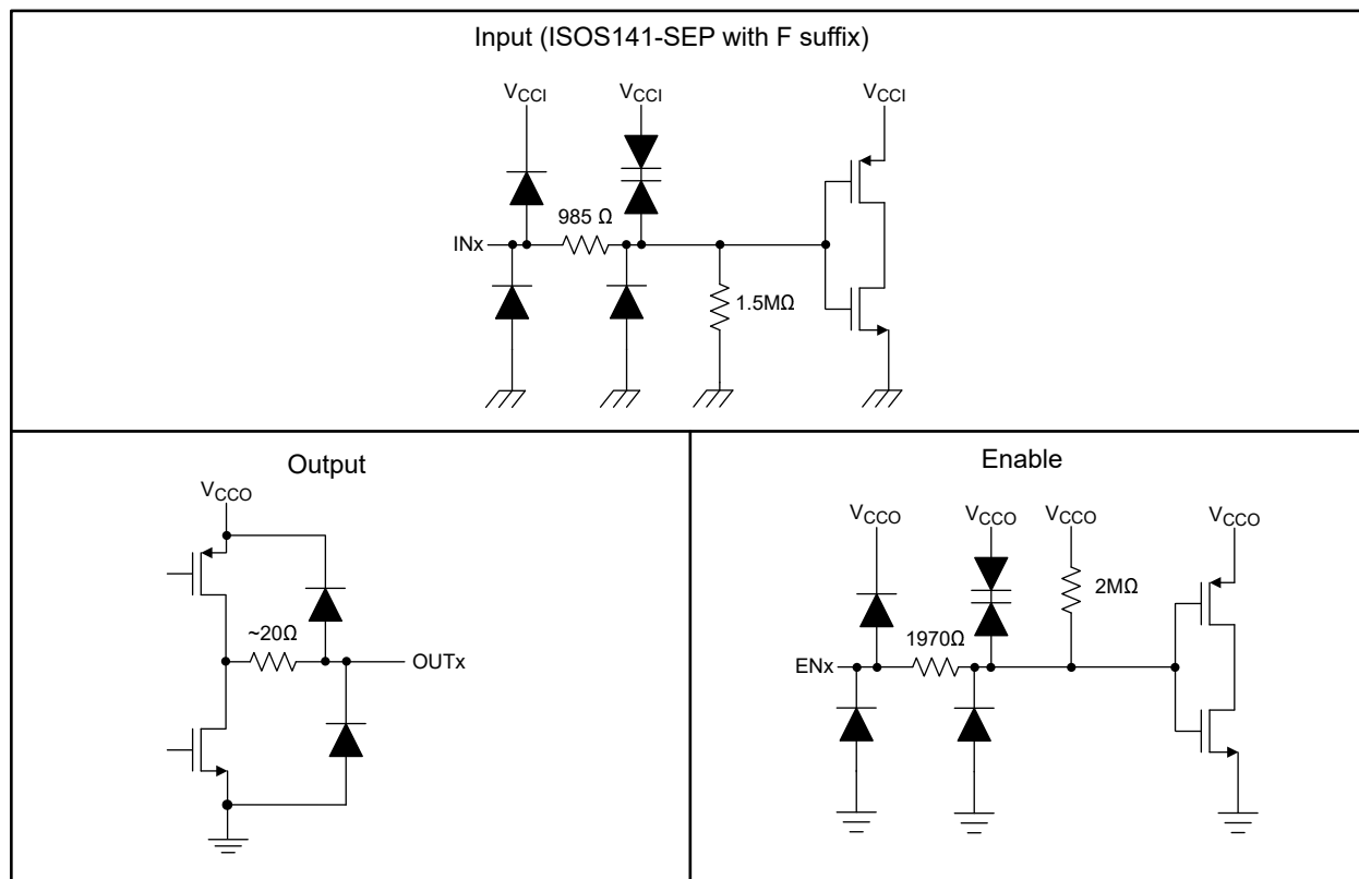
Figure 8-3. Device I/O Schematics
