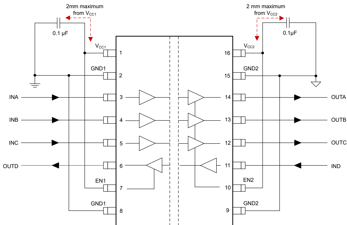
Figure 9-2. Typical ISOS141-SEP Circuit Hook-up
