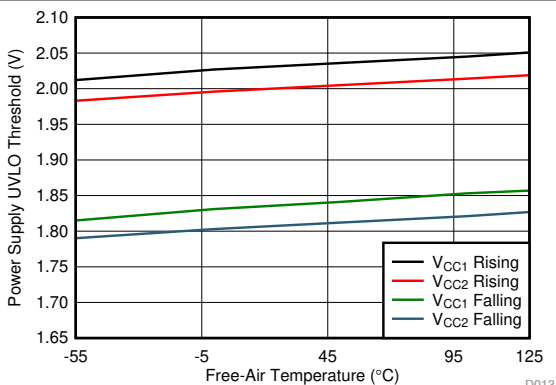
Figure 5-7. Power Supply Undervoltage Threshold vs Free-Air Temperature
