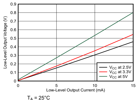
Figure 5-6. Low-Level Output Voltage vs Low-Level Output Current
