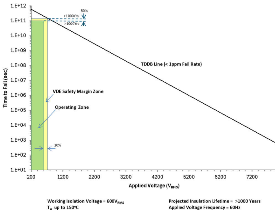
Figure 9-7. Insulation Lifetime Projection Data
