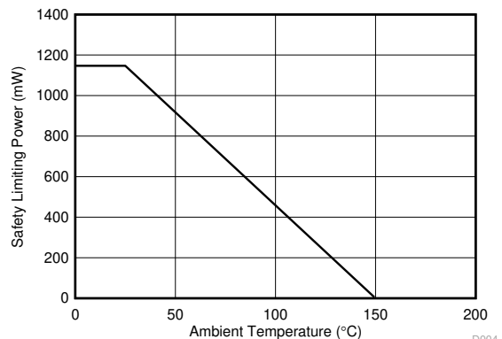
Figure 5-2. Thermal Derating Curve for Safety Limiting Power for DBQ-16 Package
