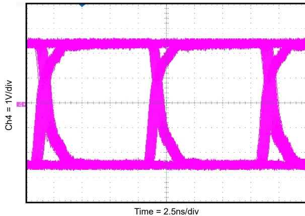
Figure 9-3. Eye Diagram at 100Mbps PRBS 2^{16} - 1 , 5V and 25°C
