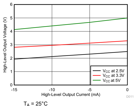
Figure 5-5. High-Level Output Voltage vs High-level Output Current
