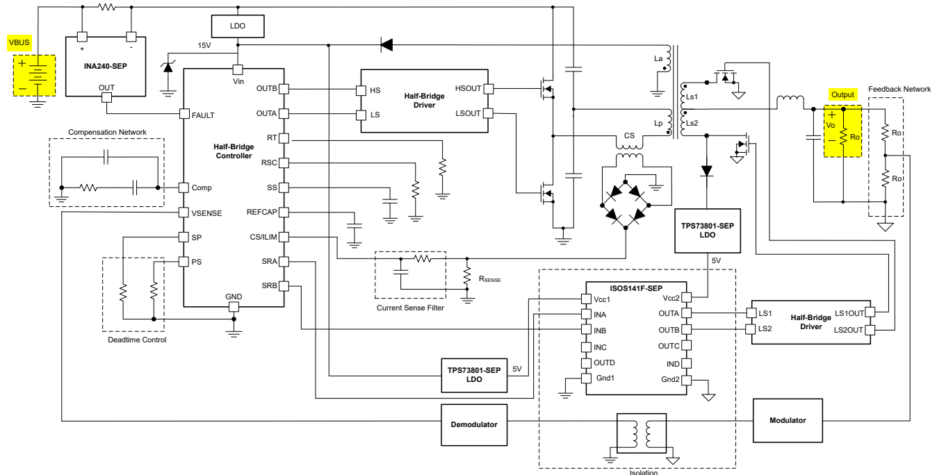
Figure 9-1. Isolated 75V to 5V 50W GaN-Based Half-Bridge Topology
