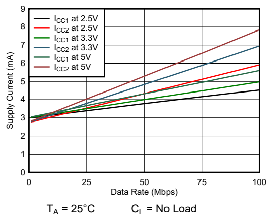
Figure 5-4. Supply Current vs Data Rate (With No Load)
