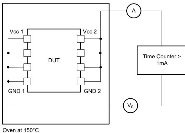
Figure 9-6. Test Setup for Insulation Lifetime Measurement
