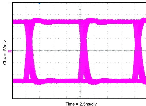
Figure 9-5. Eye Diagram at 100Mbps PRBS 2^{16} - 1 , 2.5V and 25°C
