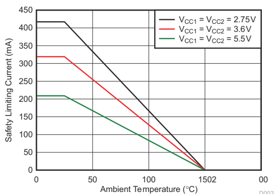
Figure 5-1. Thermal Derating Curve for Safety Limiting Current for DBQ-16 Package
