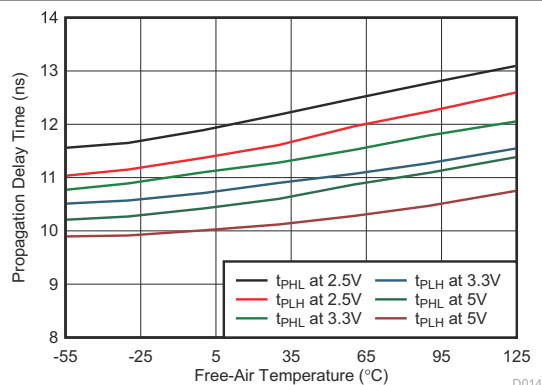
Figure 5-8. Propagation Delay Time vs Free-Air Temperature
