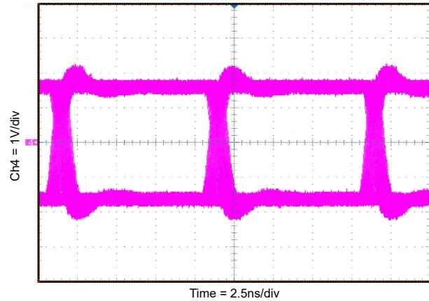
Figure 9-4. Eye Diagram at 100Mbps PRBS 2^{16} - 1 , 3.3V and 25°C
