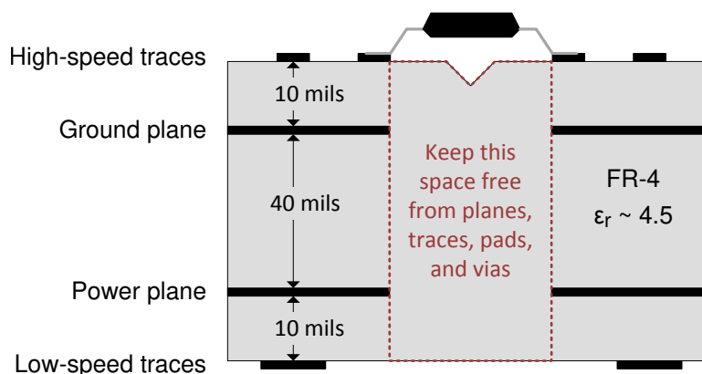
Figure 9-8. Layout Example Schematic
