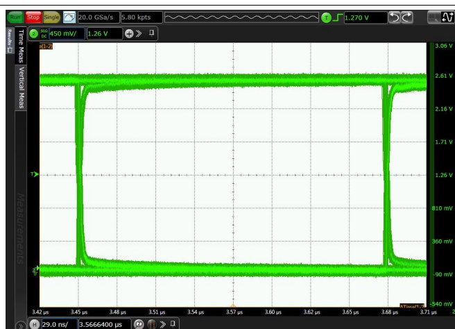
Figure 21. Eye Diagram at 4 Mbps PRBS 2^{16} - 1 , 2.5 V and 25°C
