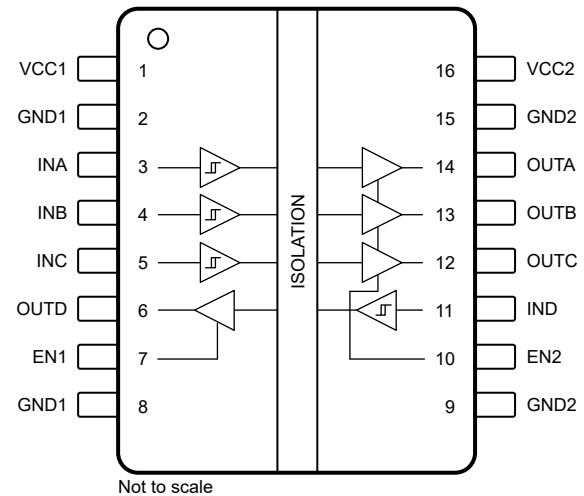
Figure 5-2. ISO6041H and ISO6041L Top View
