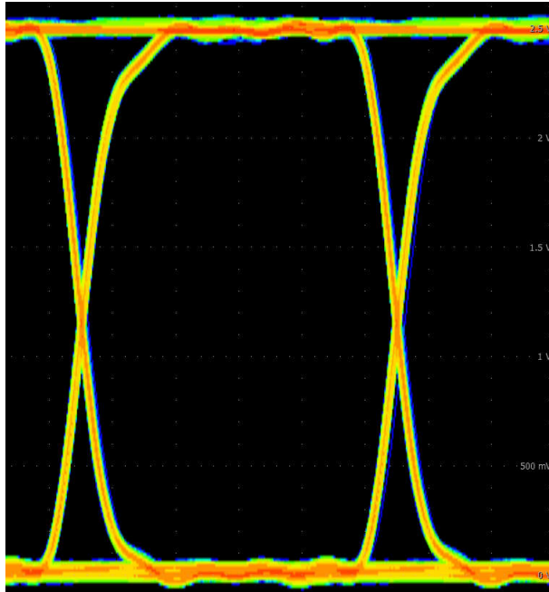
Figure 9-6. ISO604x Eye Diagram at 200Mbps PRBS 2^{16} - 1 , 2.5V and 25°C
