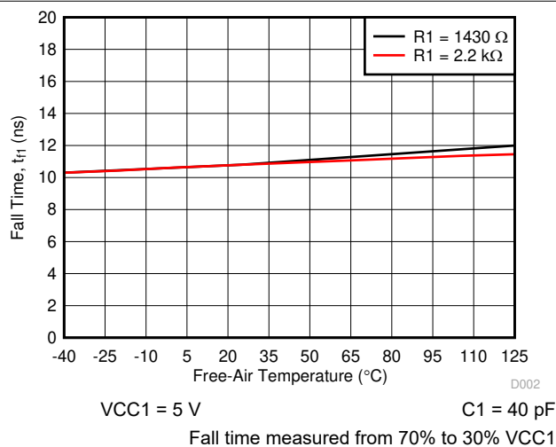
Figure 6-5. Side 1: Output Fall Time vs Free-air Temperature
