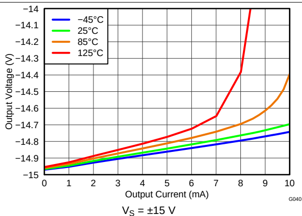
Figure 40. Negative Output Voltage Swing vs Output Current
