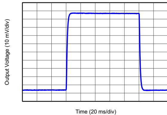
Figure 46. Small-Signal Response
