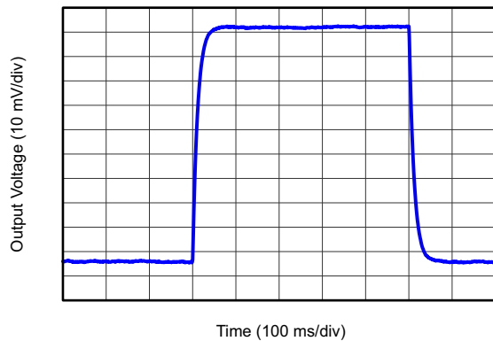
Figure 45. Small-Signal Response
