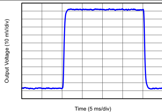
Figure 44. Small-Signal Response
