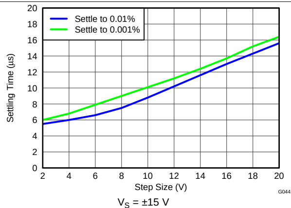
Figure 42. Settling Time vs Step Size
