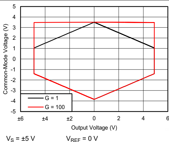
Figure 8-6. Input Common-Mode Voltage vs Output Voltage
