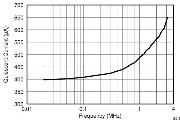
Figure 6-17. Active I_Q vs. I^2\text{C} Clock Frequency
