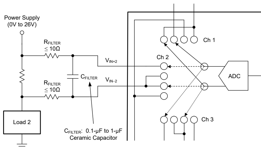
Figure 7-8. INA3221-Q1 With Input Filtering
