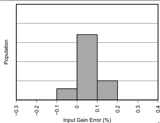
Figure 6-10. Bus Input Gain Error Production Distribution
