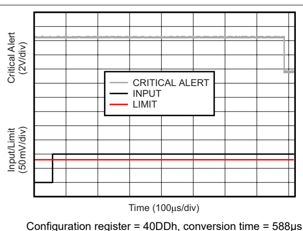
Figure 9-3. Critical Alert Response for 588 \mu s Conversion Time
