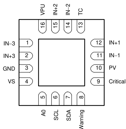
Figure 5-1. RGV Package 16-Pin VQFN Top View
