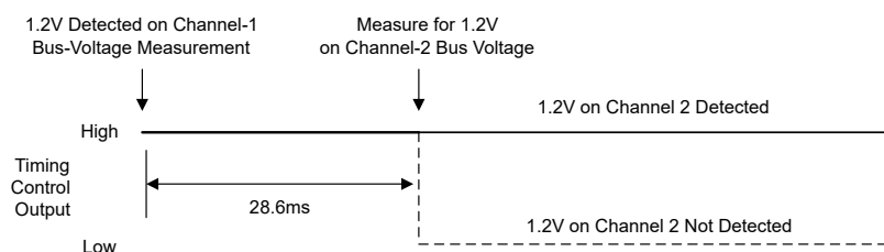
Figure 7-4. Timing Control State Diagram
