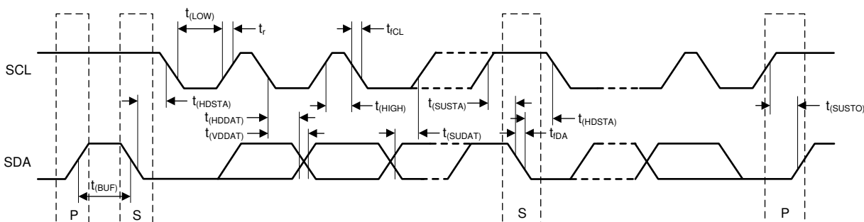
Figure 7-13. Bus Timing
