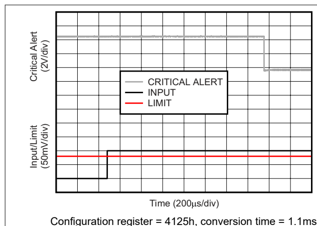
Figure 9-2. Critical Alert Response for 1.1ms Conversion Time
