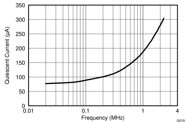
Figure 6-18. Shutdown I_Q vs. I^2\text{C} Clock Frequency
