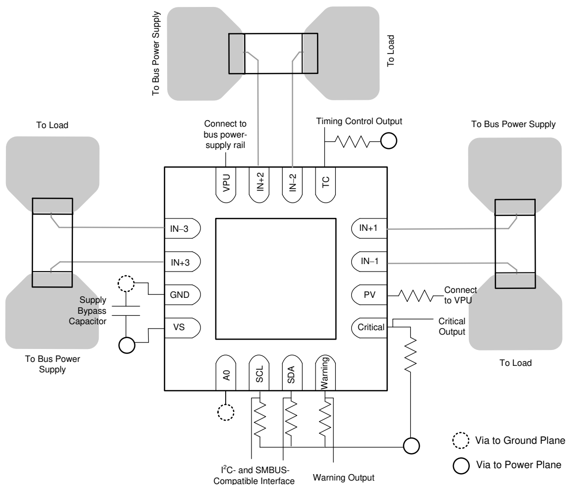
Figure 9-4. Layout Example
