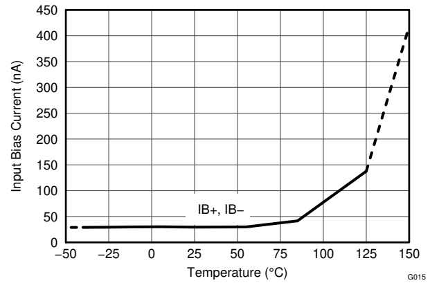
Figure 6-14. Input Bias Current vs. Temperature (Shutdown)
