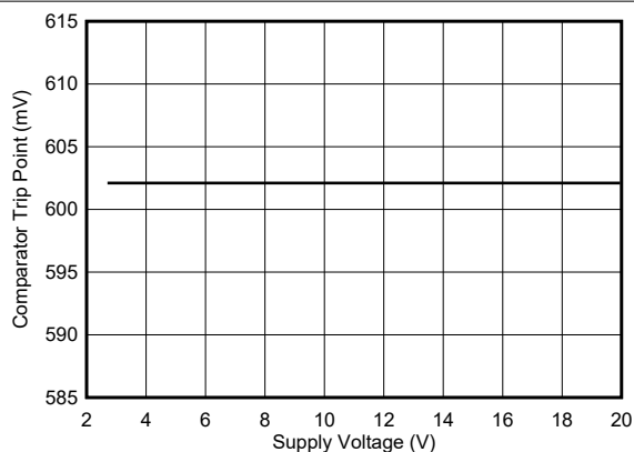
Figure 6-35. Comparator Trip Point vs Supply Voltage
