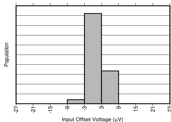
Figure 6-4. INA310A4 Input Offset Production Distribution
