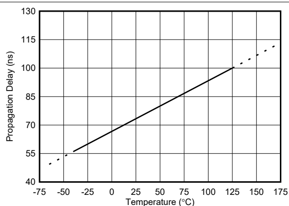
Figure 6-39. Comparator Propagation Delay vs Temperature
