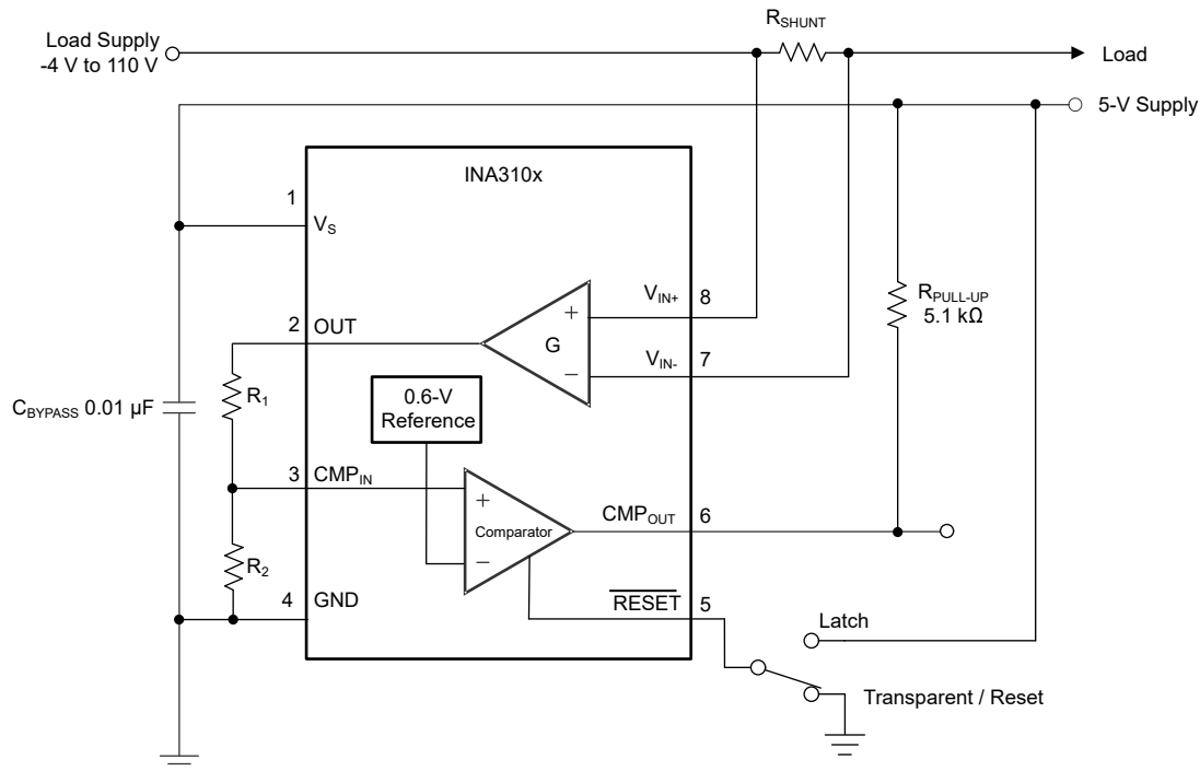
Figure 7-4. INA310 Basic Connections
