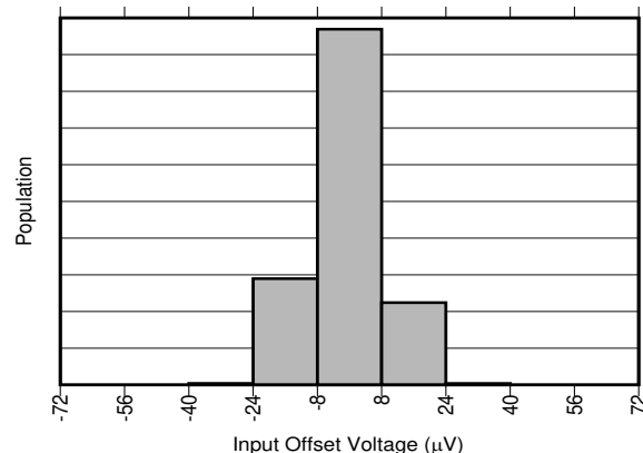
Figure 6-2. INA310A2 Input Offset Production Distribution
