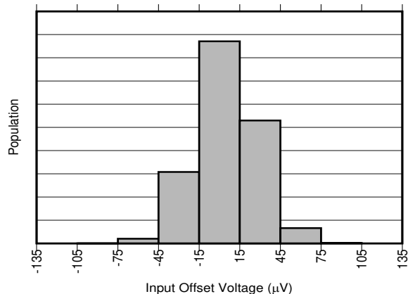
Figure 6-1. INA310A1 Input Offset Production Distribution
