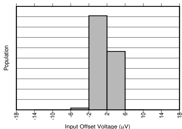
Figure 6-5. INA310A5 Input Offset Production Distribution
