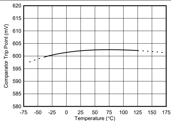
Figure 6-36. Comparator Trip Point vs Temperature
