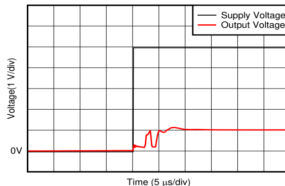
Figure 6-32. Start-Up Response
