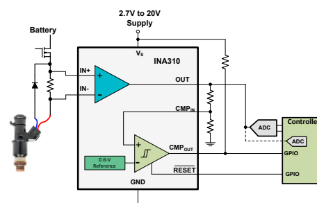
Typical Application
