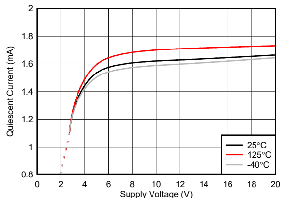
Figure 6-28. Quiescent Current vs Supply Voltage
