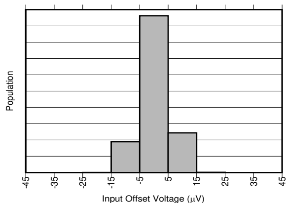
Figure 6-3. INA310A3 Input Offset Production Distribution
