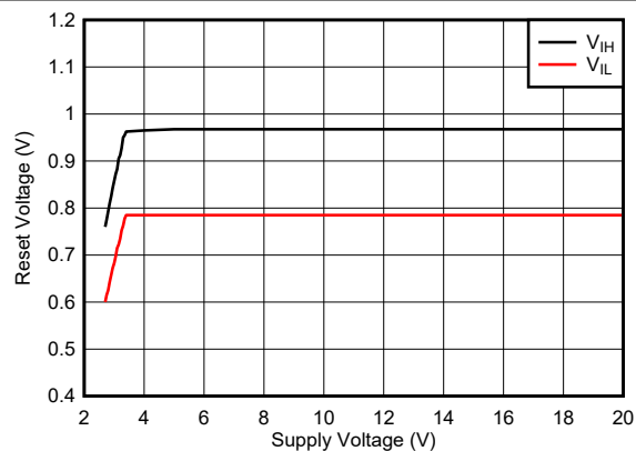
Figure 6-38. Comparator Reset Voltage vs Supply Voltage
