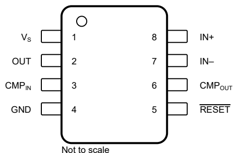
Figure 5-1. INA310x: DGG Package 8-Pin VSSOP Top View
