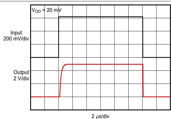
Figure 6-40. Comparator Propagation Delay
