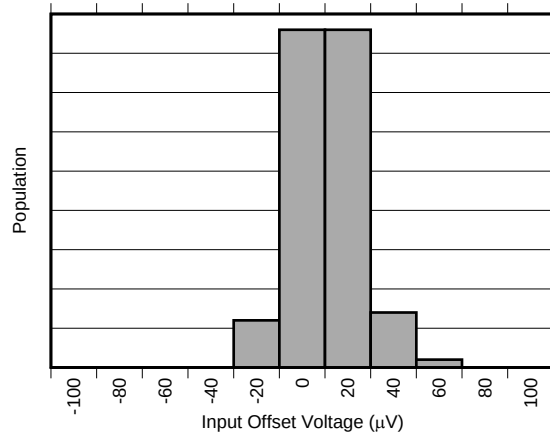
Figure 1. Input Offset Voltage Distribution (INA30xA1)
