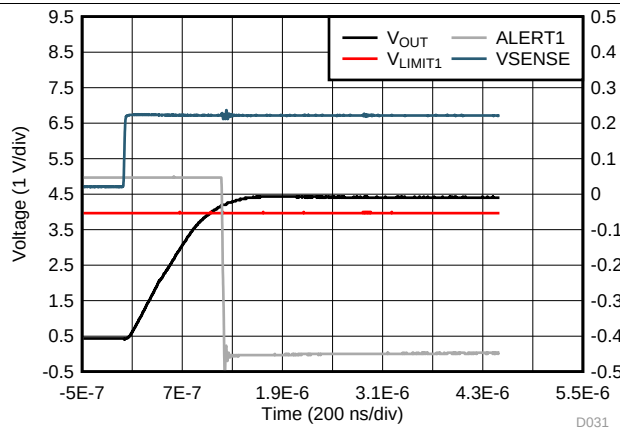
Figure 31. Comparator 1 Total Propagation Delay (INA30x)
