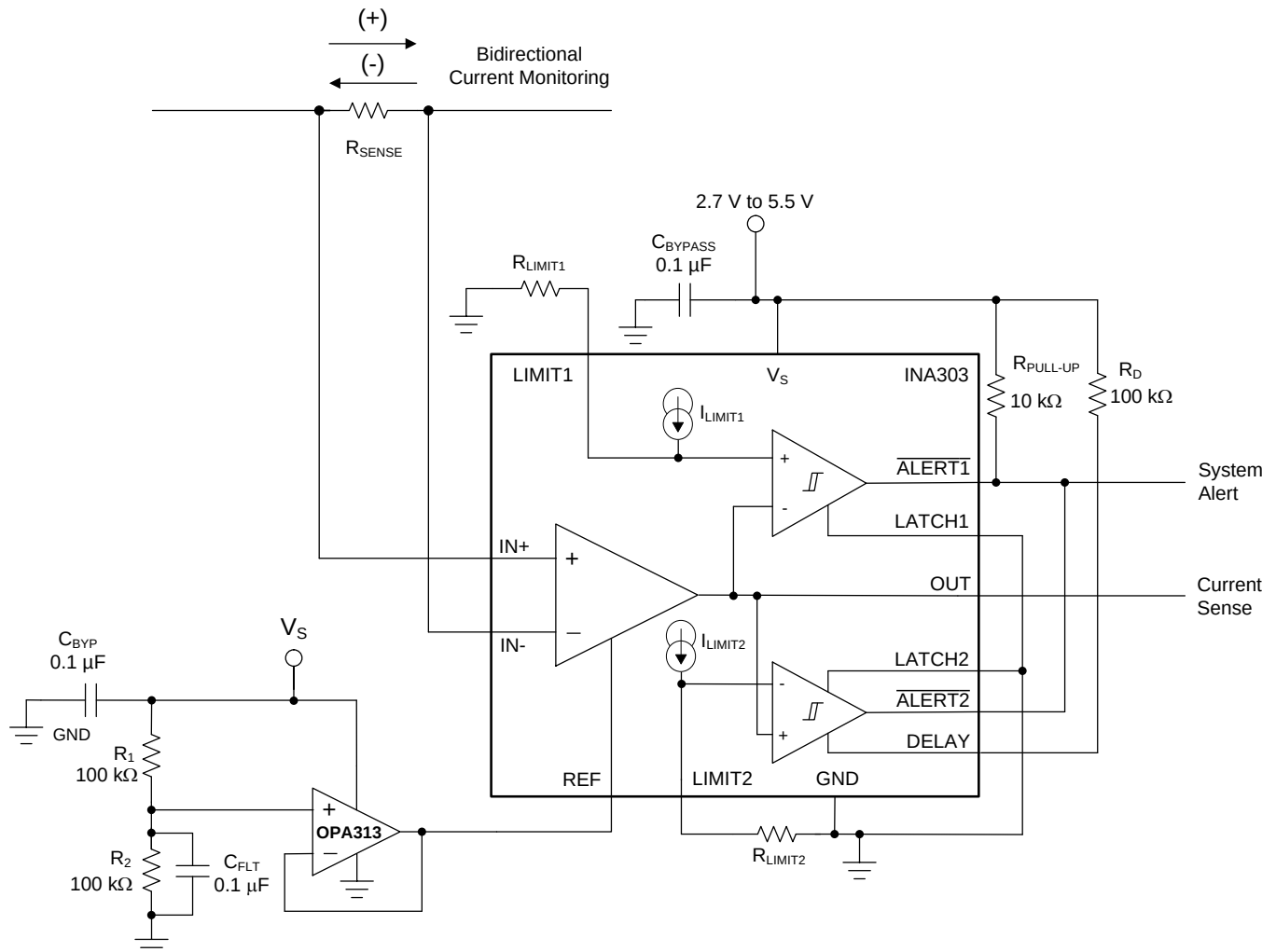
Figure 52. Bidirectional Application
