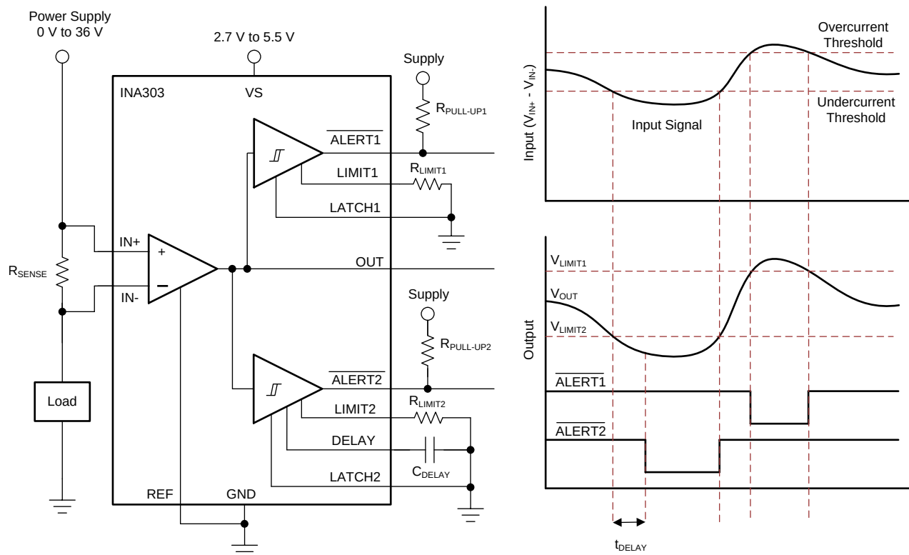
Figure 43. Out-of-Range Alert Responses for the INA303
