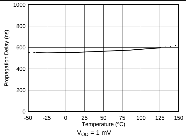
Figure 36. Comparator 1 Propagation Delay vs Temperature
