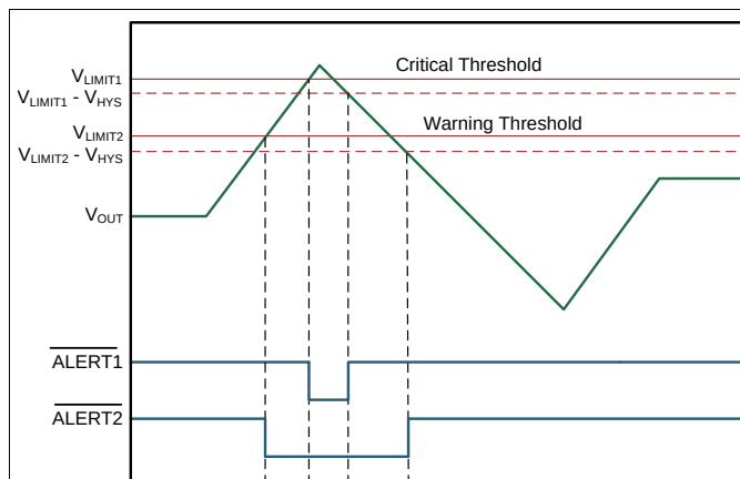
Figure 45. Comparator Hysteresis Behavior (INA302)
