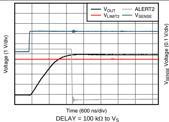
Figure 33. Comparator 2 Total Propagation Delay (INA303)
