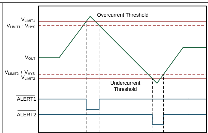
Figure 46. Comparator Hysteresis Behavior (INA303)
