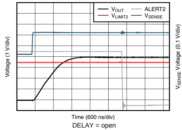
Figure 32. Comparator 2 Total Propagation Delay (INA303)
