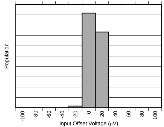
Figure 2. Input Offset Voltage Distribution (INA30xA2)
