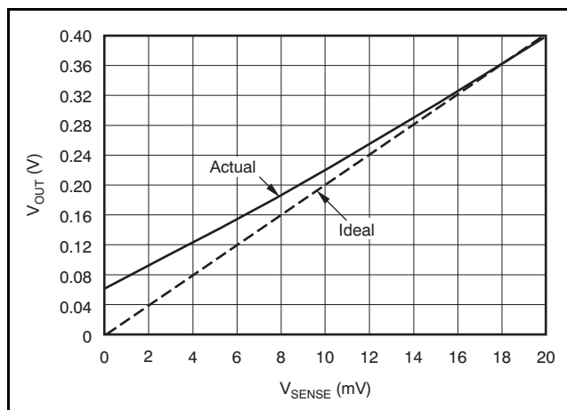
Figure 18. Example for Low V_{SENSE} Cases 1 and 3 (Gain = 20)
