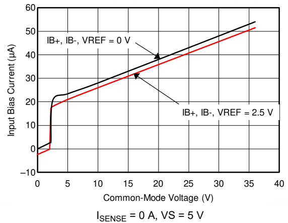
Figure 6-20. Input Bias Current vs Common-Mode Voltage (VS = 5 V)
