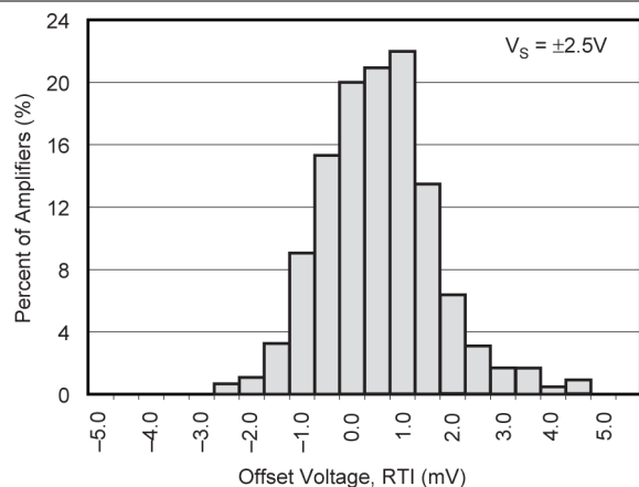
Figure 5-25. Offset Voltage Production Distribution
