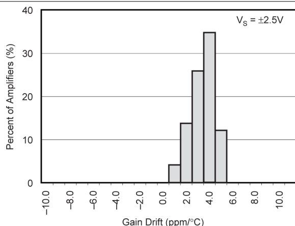
Figure 5-29. Gain Drift Production Distribution
