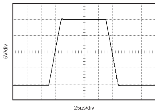
Figure 5-17. Large-Signal Step Response ( R_L = 10\text{k}\Omega , C_L = 10\text{pF} )
