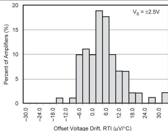
Figure 5-27. Offset Voltage Drift Production Distribution
